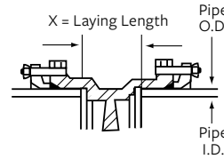
INSTALLATION DIAGRAM
