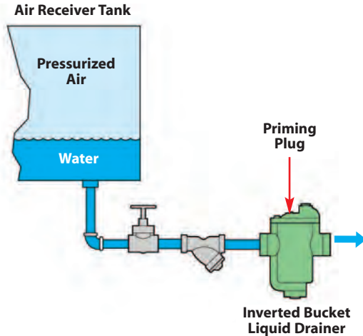
Figure 3 Draining Condensate from a Receiver with an Inverted Bucket Style Liquid Drainer
